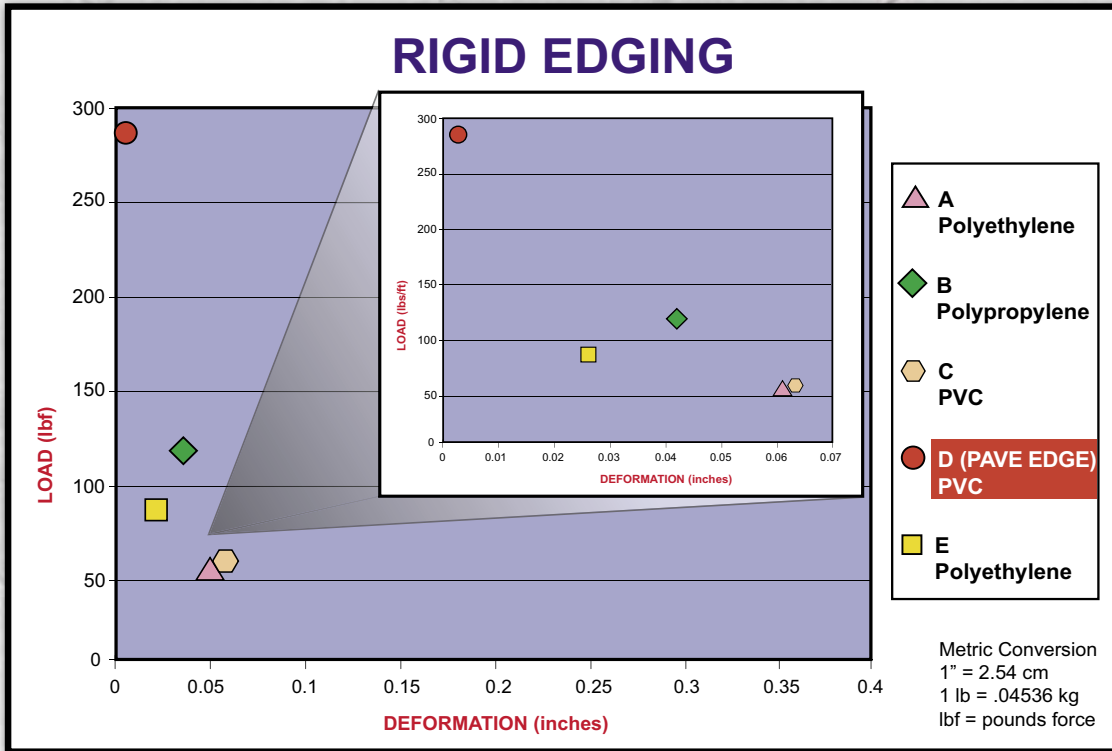
This chart shows the correlation between Deformation and Load on the rigid edging.
