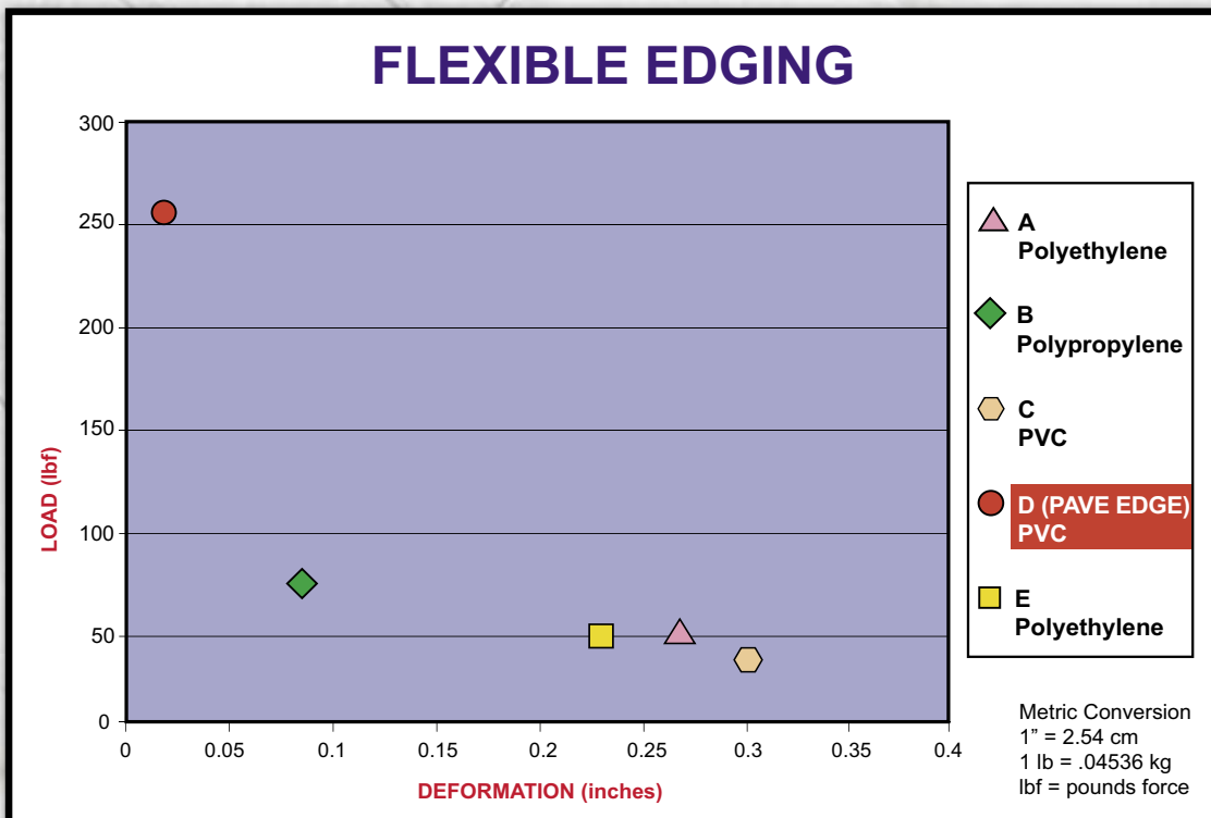
This chart shows the correlation between Deformation and Load on the flexible edgings.
